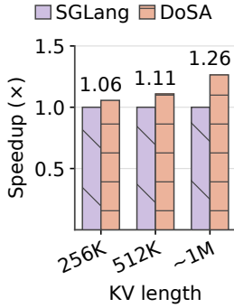
Figure 5: Decoding Indexer speedup over SGLang.
