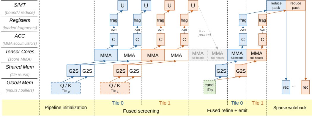
Figure 3: Data flow through screening, refinement, and sparse writeback. Blue and orange denote successive tiles, with key loading overlapped with computation. SIMT threads evaluate bounds U using on-chip accumulators (ACC); gray MMA blocks indicate pruned full-head computation. Candidate IDs feed refinement and sparse writeback. G2S and A2R denote global-to-shared and accumulator-to-register transfers.
