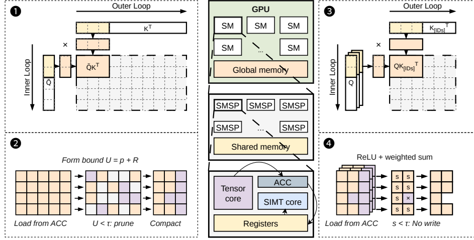
Figure 2: DOSA execution overview, read in order ①–④: ① screening dot products; ② bound evaluation, pruning, and candidate compaction; ③ full-head dot products for survivors; ④ original-score reduction and sparse writeback. Tensor Cores execute stages ① and ③; SIMT threads execute stages ② and ④ using on-chip accumulators (ACC), with gray and purple data tiles indicating avoided computation and writeback, respectively. The center sketches GPU resources; seed initialization and final Top- K selection are omitted.
