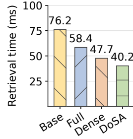
Figure 7: Screening and sparse writeback ablation.
