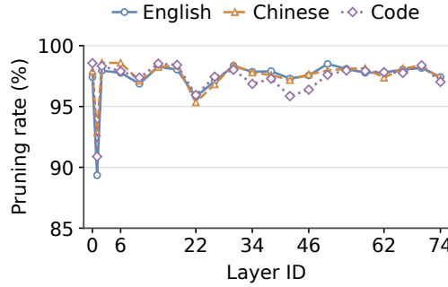
Figure 6: Certificate pruning rates across GLM-5.2 layers, averaged within each input domain.
