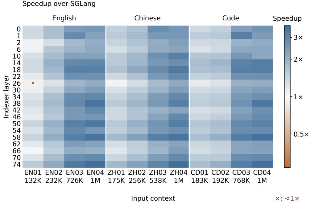
Figure 11: Per-layer retrieval speedup over SGLang for the final 32K queries. Columns identify inputs and context lengths; rows identify indexer layers. Crosses mark cells slower than the baseline. The logarithmic color scale is centered at 1\times .
