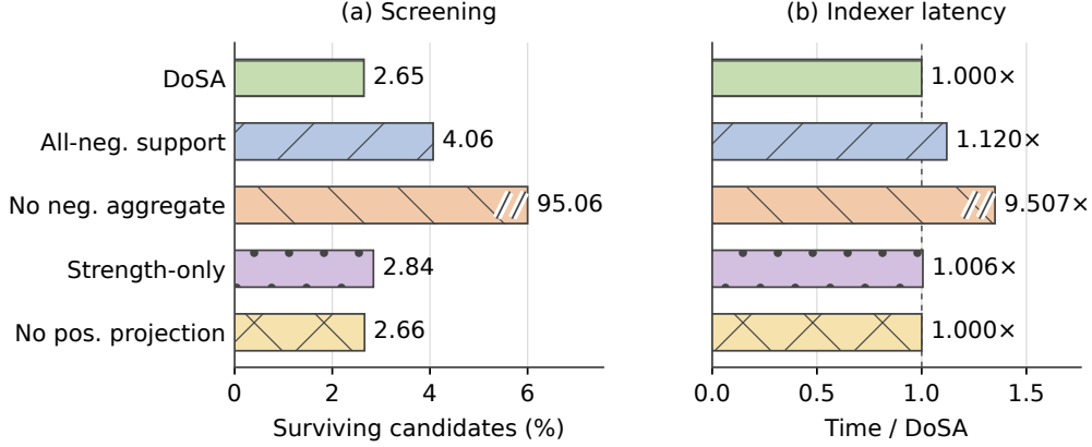
Figure 9: Effects of certificate components on screening and Indexer latency. Bars show the mean candidate survival rate and geometric mean latency relative to DoSA. Breaks mark bars beyond the displayed range; annotations give their measured values.
