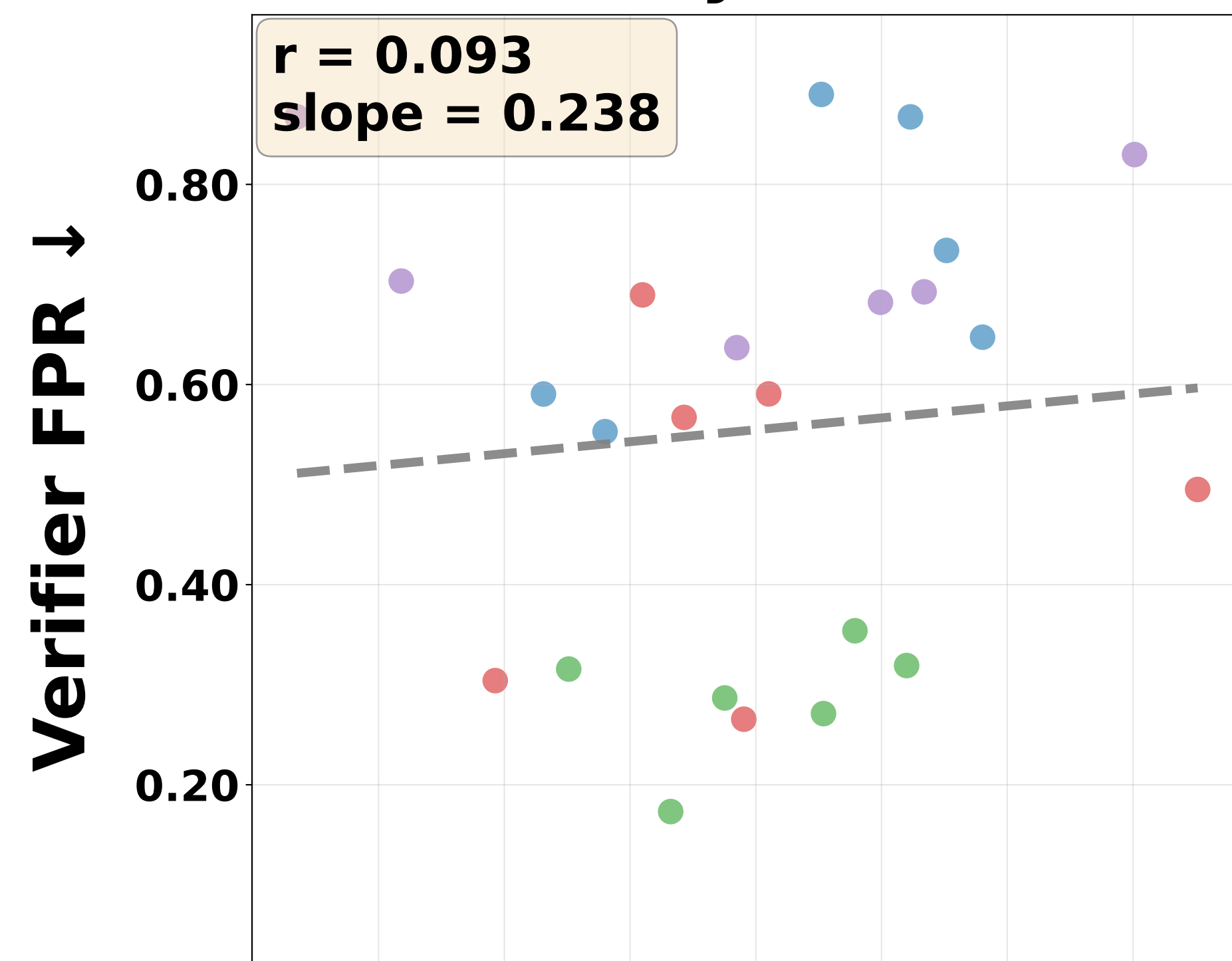
Intra-Family Verification
