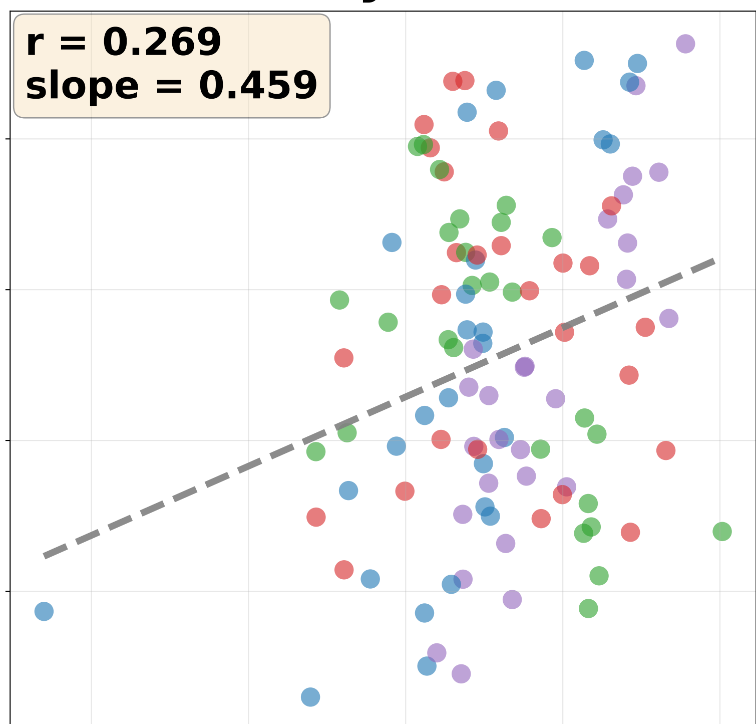
Cross-Family Verification
