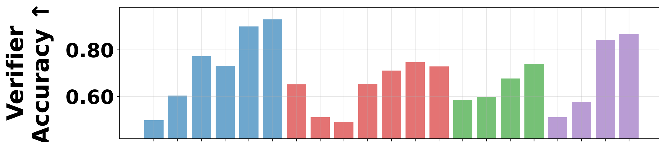
Self-Verification
