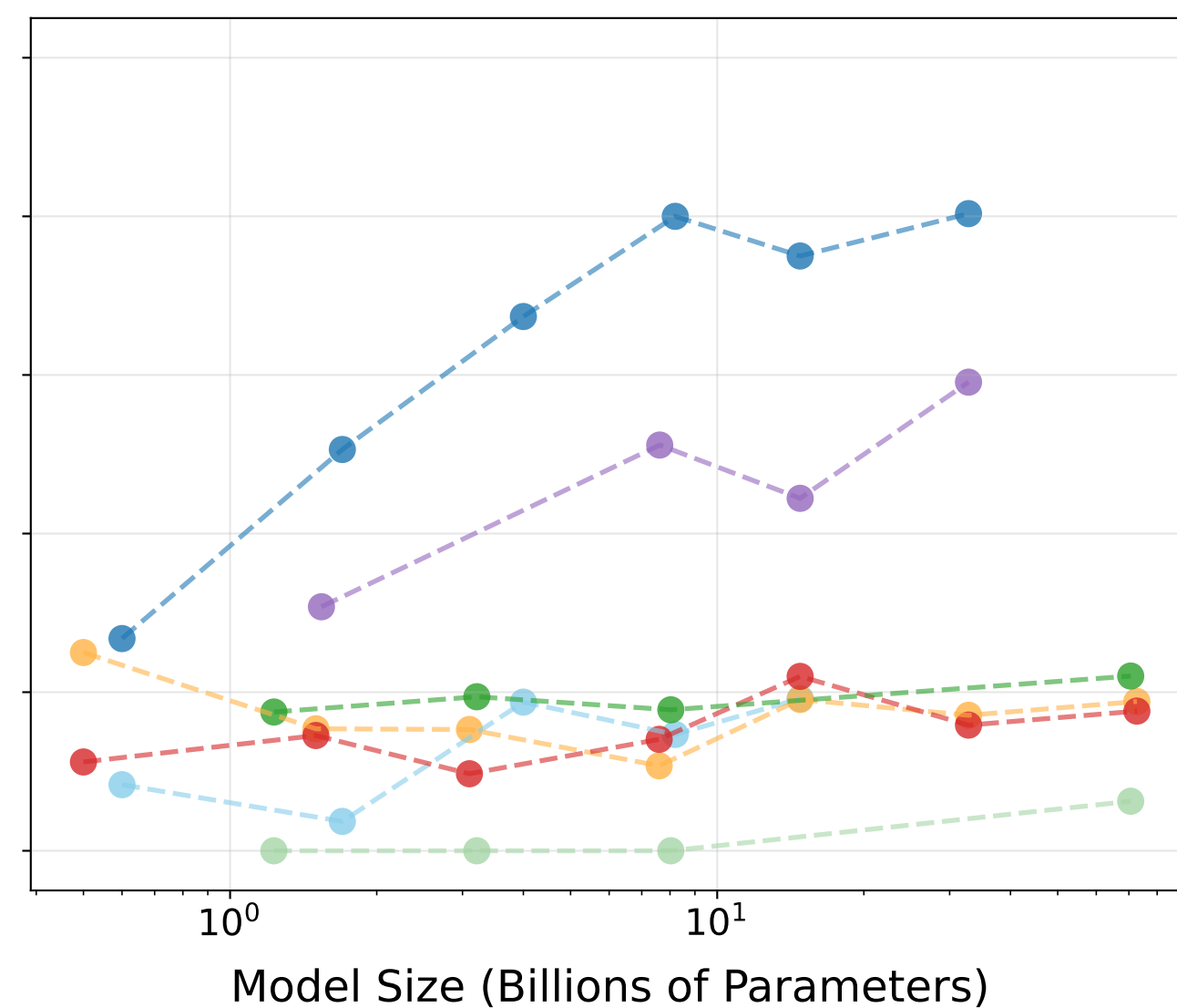
GPQA Solver Accuracy ↑
