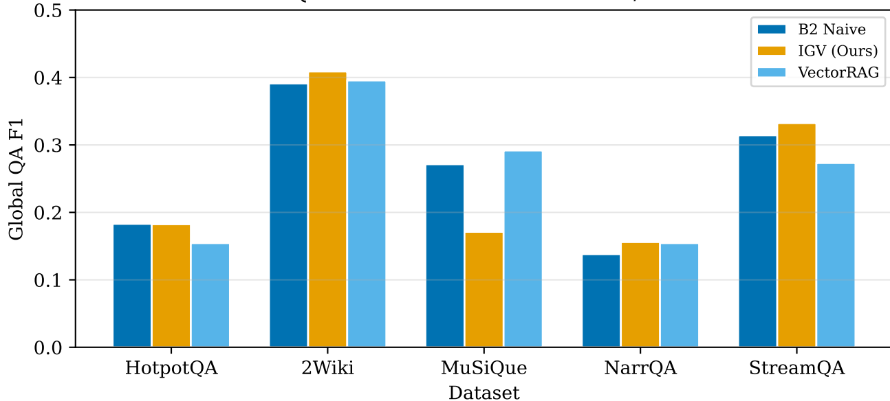
Global QA: IGV beats VectorRAG on 4/5 datasets
