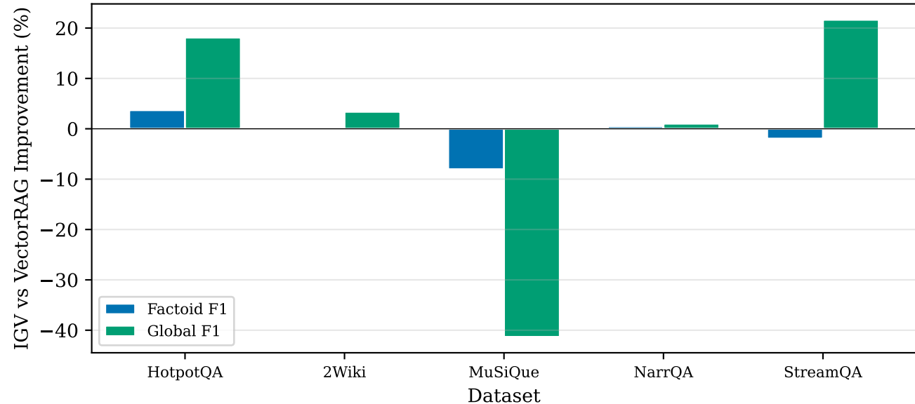
IGV improvement over VectorRAG
