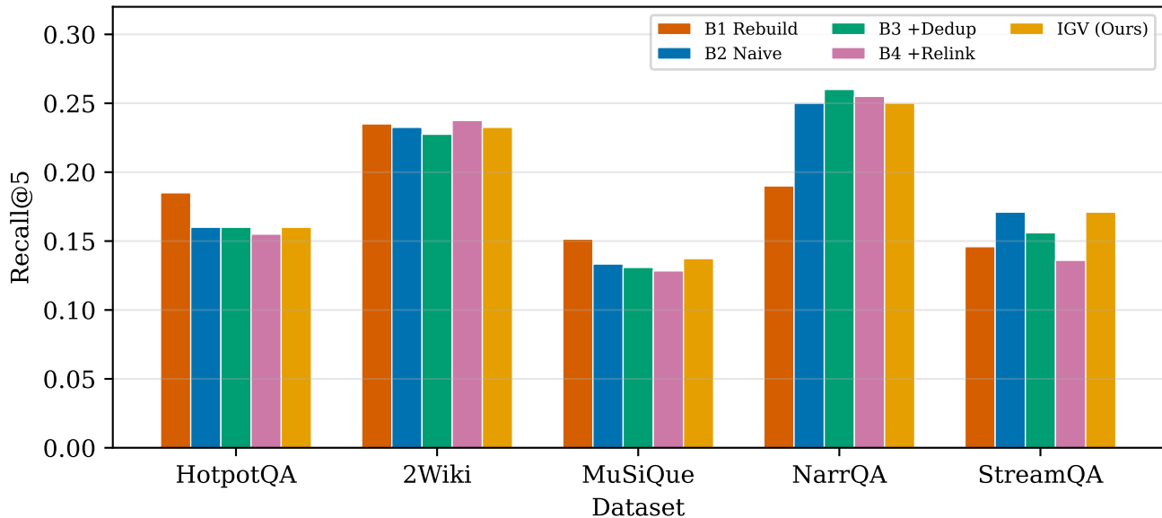
Recall@5 at Final Stage (100 questions)
