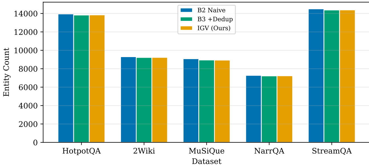
Entity Count at Final Stage
