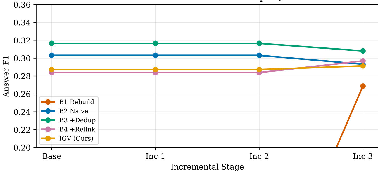
Answer F1 Evolution on HotpotQA
