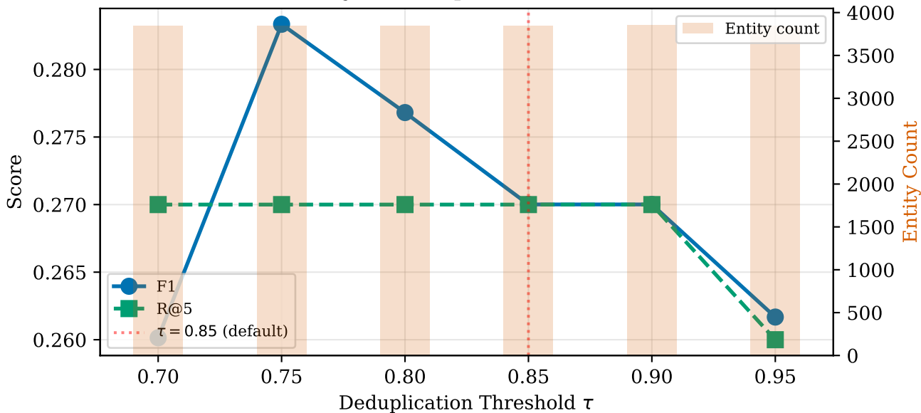
Sensitivity to Deduplication Threshold \tau
