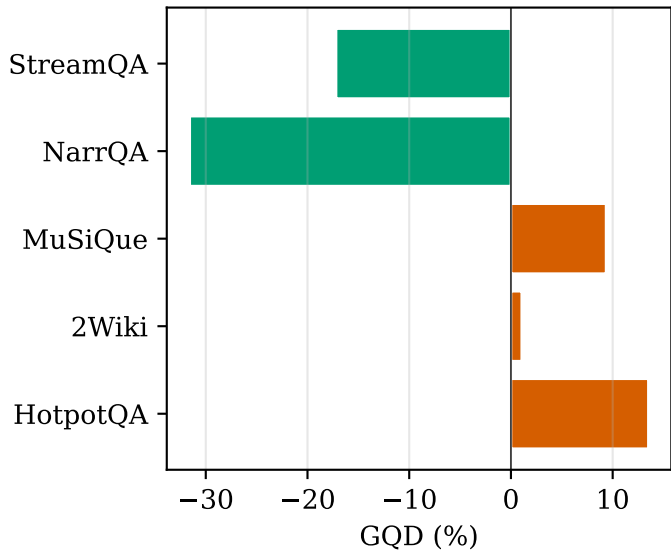
Graph Quality Degradation
