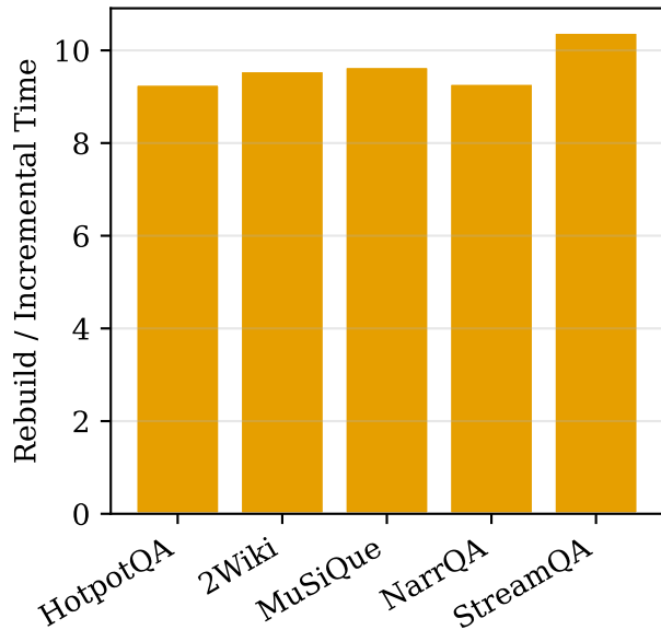
Update Efficiency Ratio (UER)
