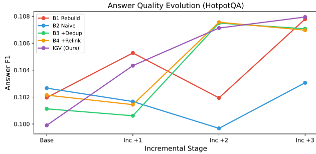
Figure 4: Answer F1 evolution on HotpotQA across incremental stages. IGV maintains quality while B2 degrades.
