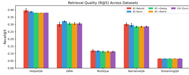
Figure 1: Recall@5 across five datasets. IGV maintains retrieval quality within 2% of full rebuild. Error bars show std over 3 seeds.
