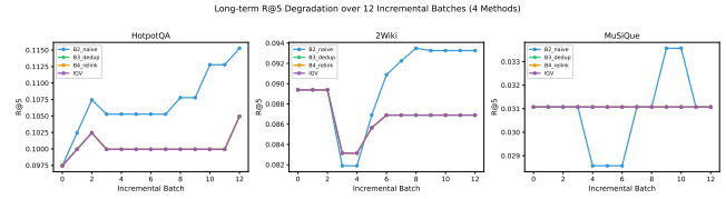
Figure 6: Long-term R@5 degradation over 12 incremental batches on three datasets (4 methods). B2 drifts significantly on HotpotQA while B3/B4/IGV remain stable.
