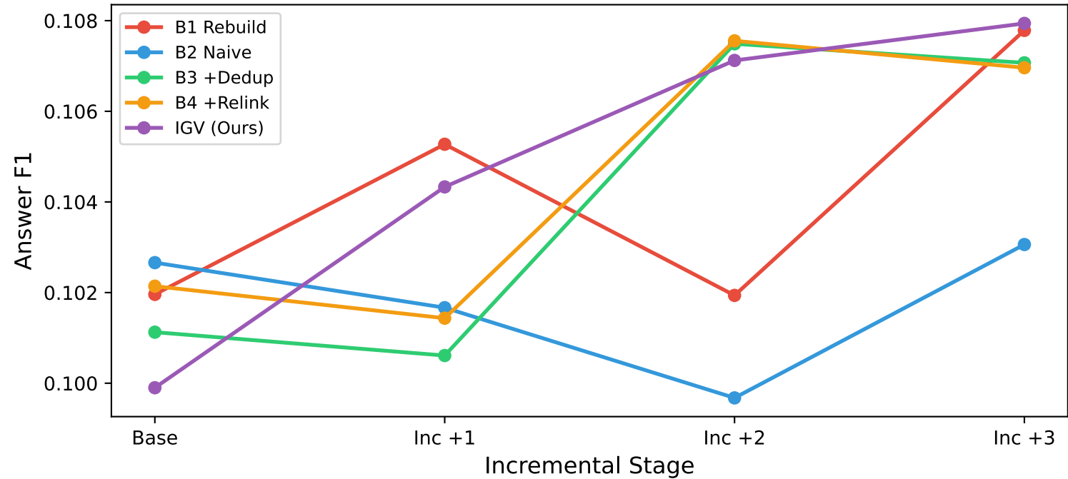
Answer Quality Evolution (HotpotQA)
