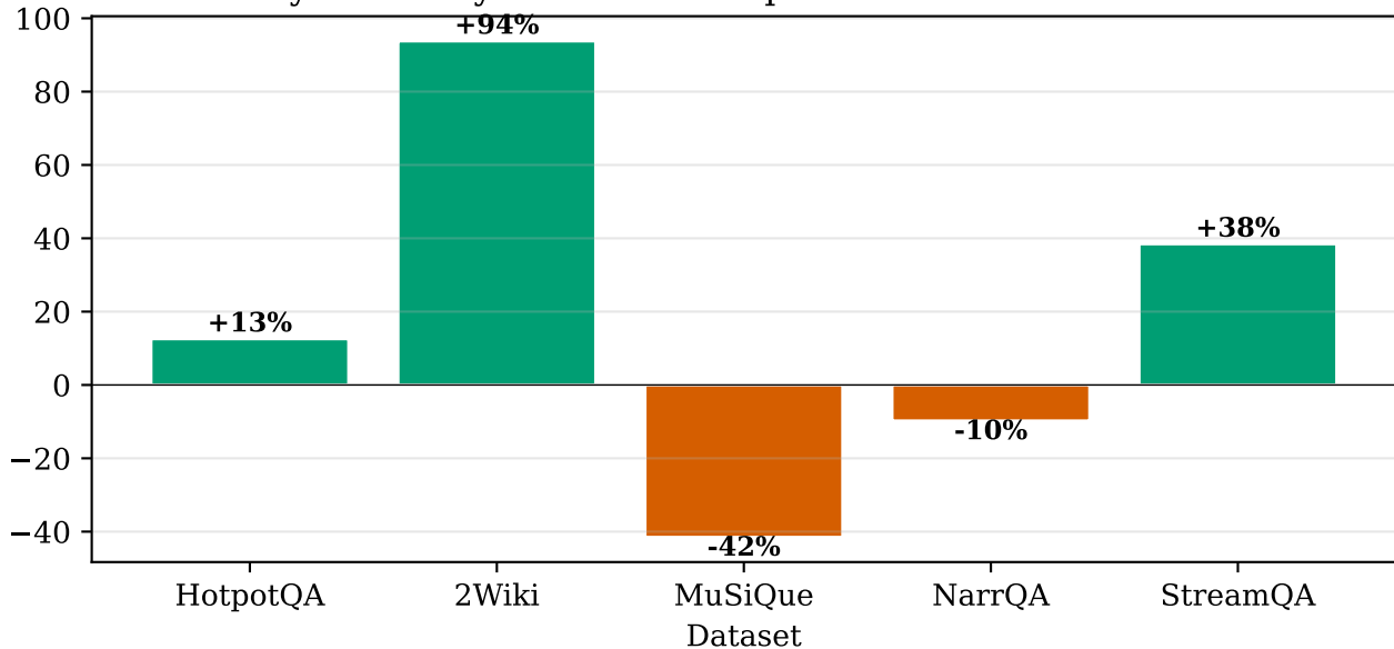
Community Summary Bonus: IGV improvement over naive incremental
