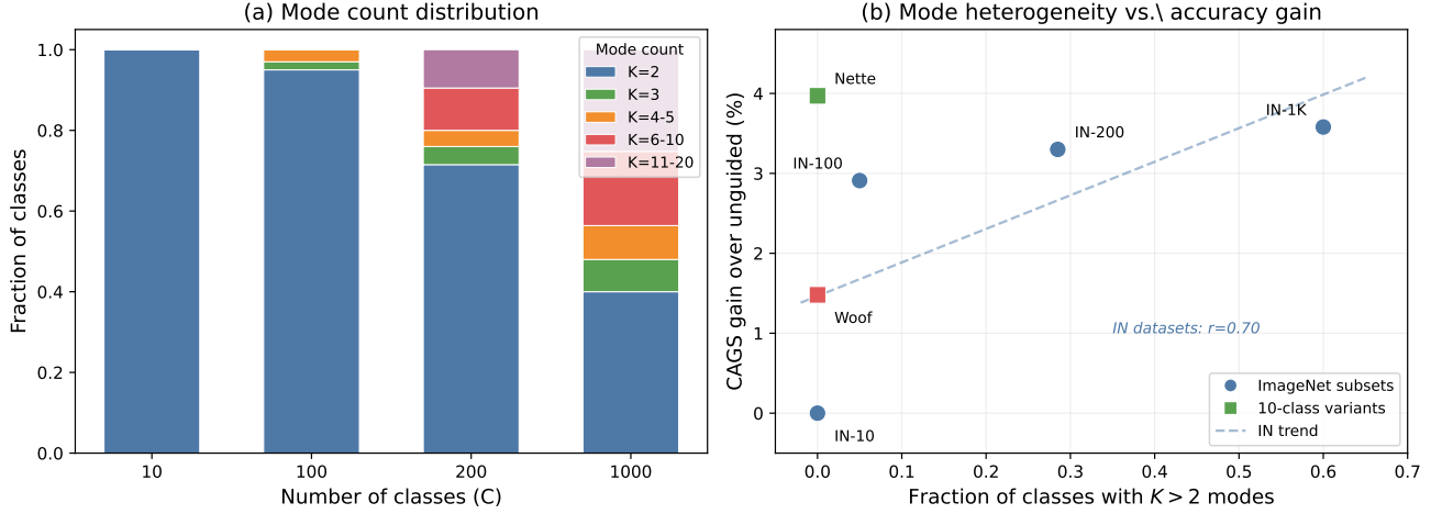
Figure 1: Quantitative validation of Theorem 1. (a) Distribution of mode counts ( K ) across ImageNet subsets with increasing class count. (b) Mode heterogeneity (fraction of classes with K > 2 ) vs. actual CAGS accuracy gain.
