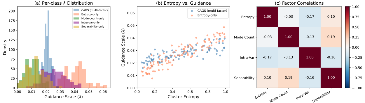
Figure 4: Guidance analysis on ImageNet-100. (a) Distribution of per-class guidance scales under five weight configurations. Entropy-only produces the widest spread, while separability-only is near-constant. (b) Cluster entropy vs. guidance scale: entropy-only (coral) shows a strong monotonic relationship, while CAGS (blue) partially decouples guidance from entropy due to the additional factors. (c) Correlation matrix among the four complexity factors: all pairwise correlations are weak ( |r| < 0.19 ), confirming they capture independent aspects of class complexity.
