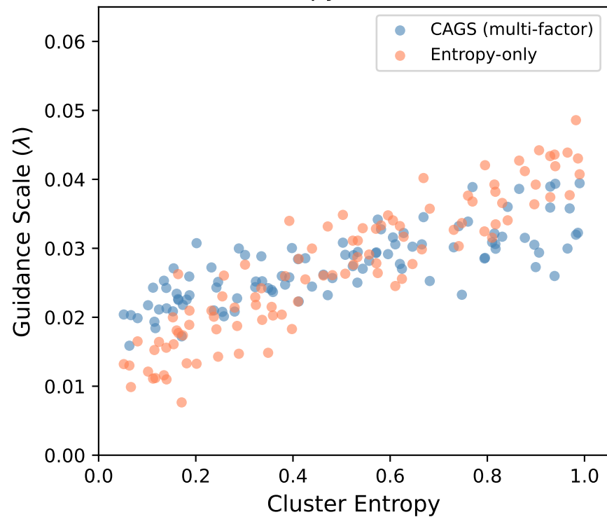
(b) Entropy vs. Guidance
