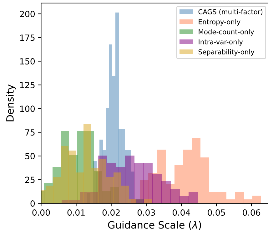
(a) Per-class \lambda Distribution
