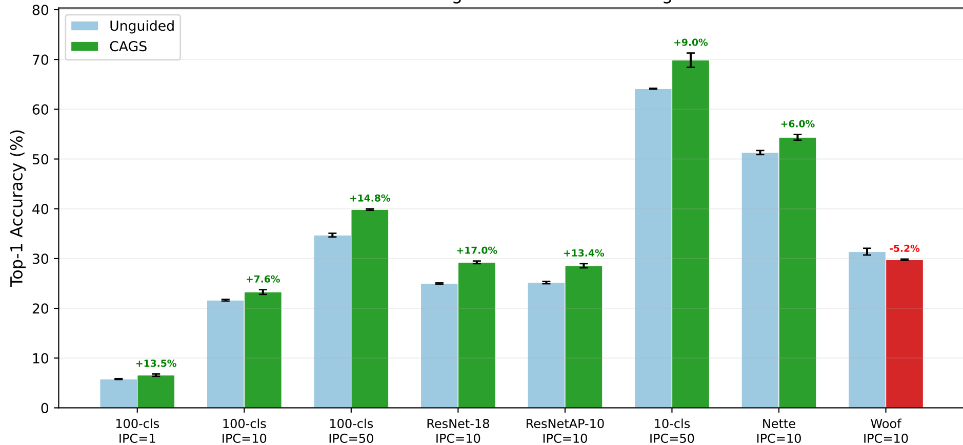
CAGS vs. Unguided Across All Settings
