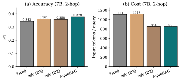
Figure 3: Ablation at 7B/2-hop. Disabling early stopping (D3) raises cost to the baseline level while lowering F1—it both cuts cost and improves accuracy in this strong-judge setting. Disabling adaptive beam (D2) keeps cost but lowers accuracy.
