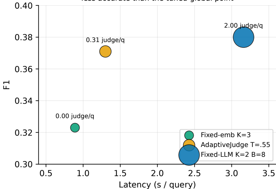
Cost--latency: adaptation is cheaper but still less accurate than the tuned global point
