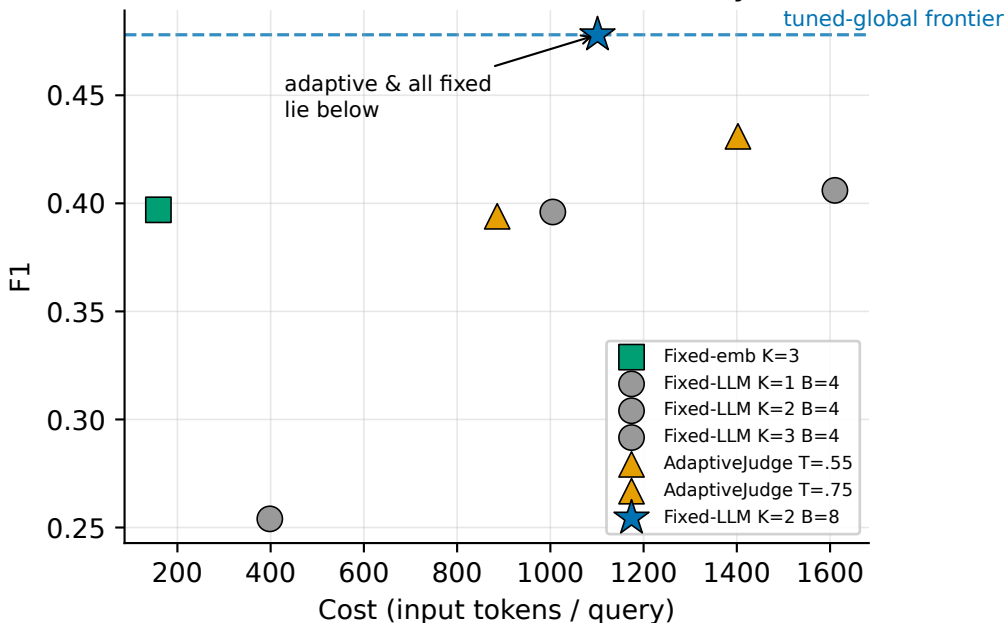
MetaQA mixed stream (7B): accuracy--cost
