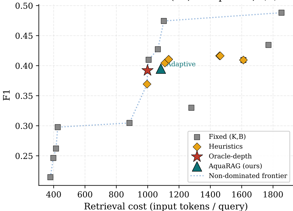
Mixed-stream Pareto frontier (7B, 240 queries, 1/2/3-hop)
