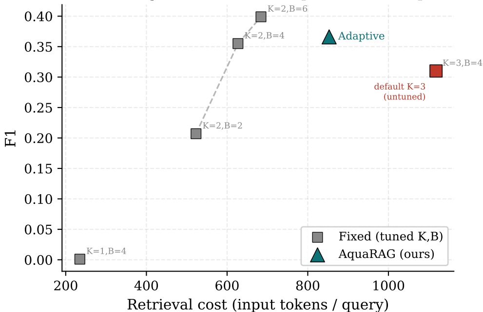
Tuned fixed-budget frontier vs. Adaptive (7B, 2-hop, n=200)
