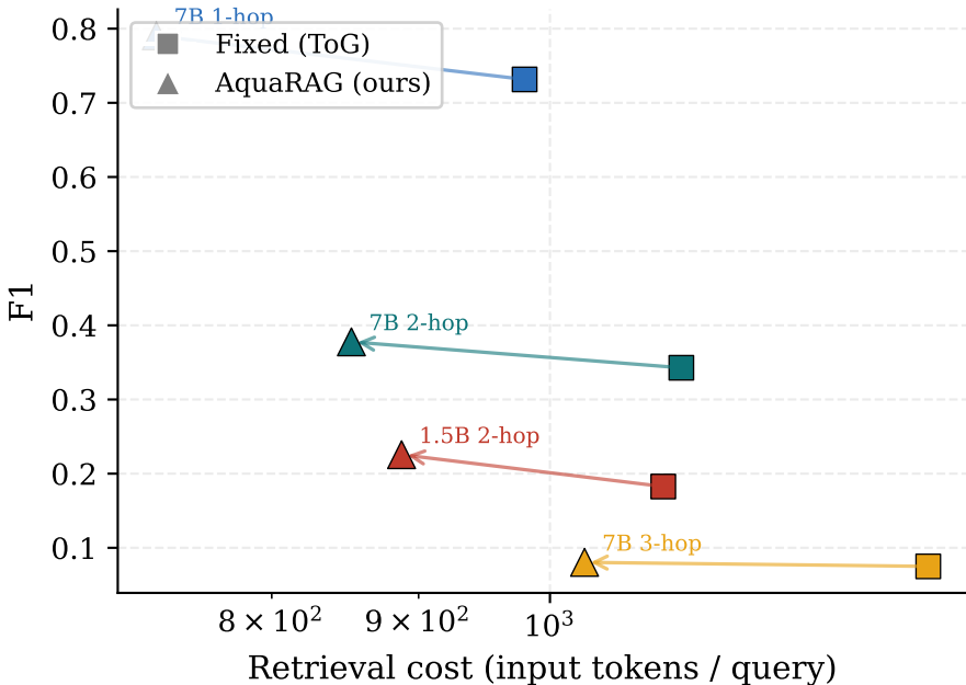
Pareto frontier: accuracy vs. cost
