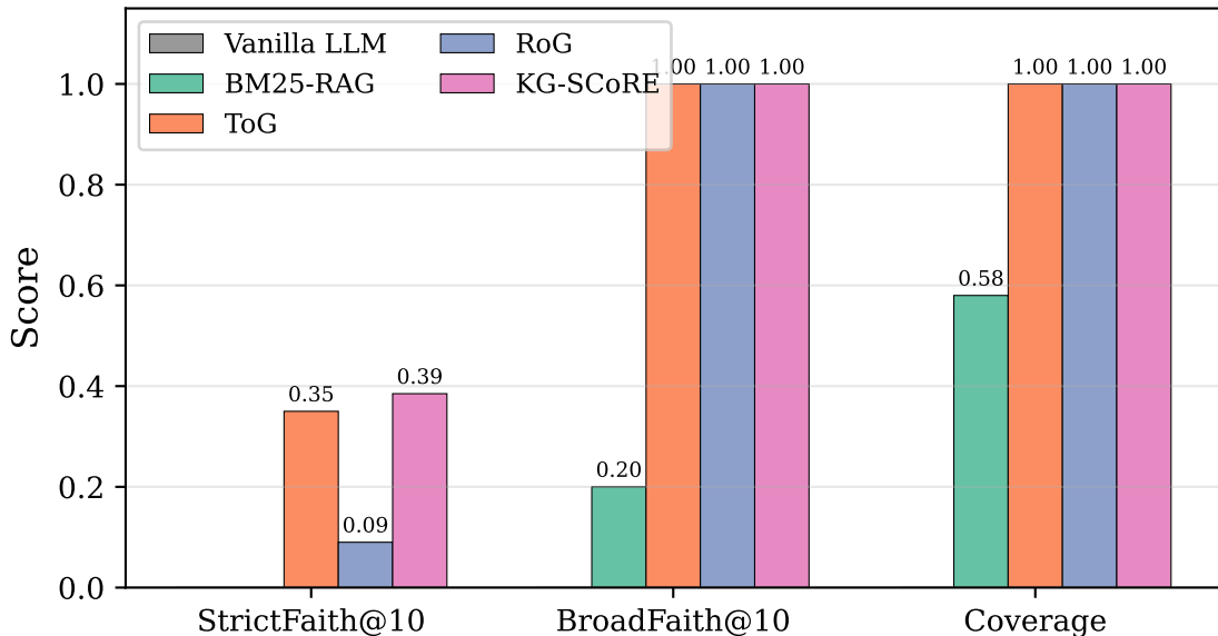
Fair Faithfulness Comparison (10 pairs, post-hoc path extraction)
