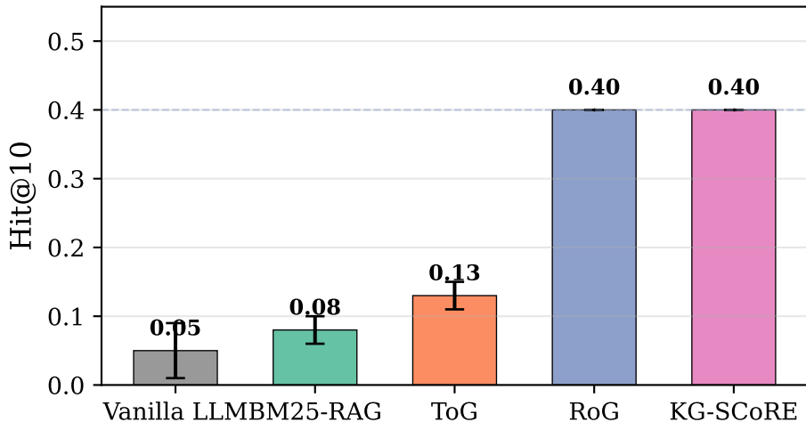
LBD Re-discovery Hit@10 (n=60, 3 seeds \times 20 pairs)
