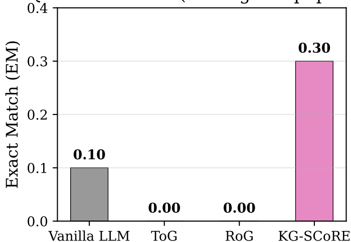
KGQA Performance (10 single-hop questions)
