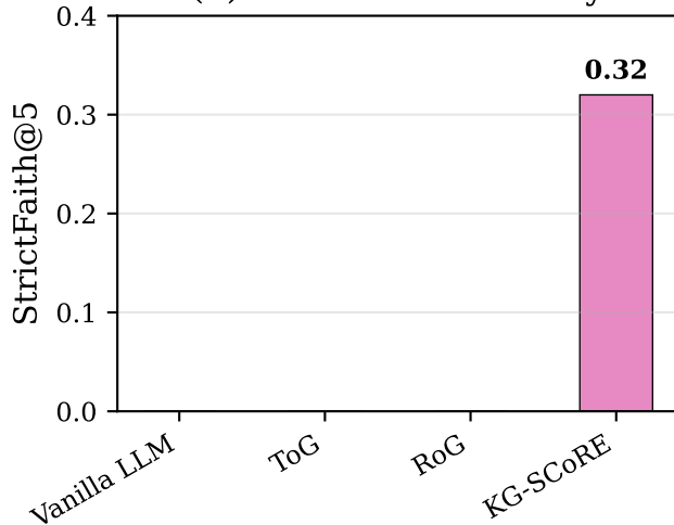
(b) Answer Traceability
