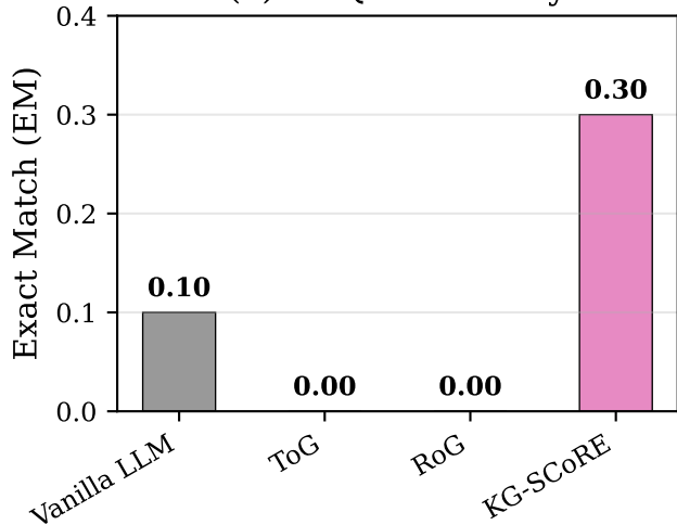
(a) KGQA Accuracy
