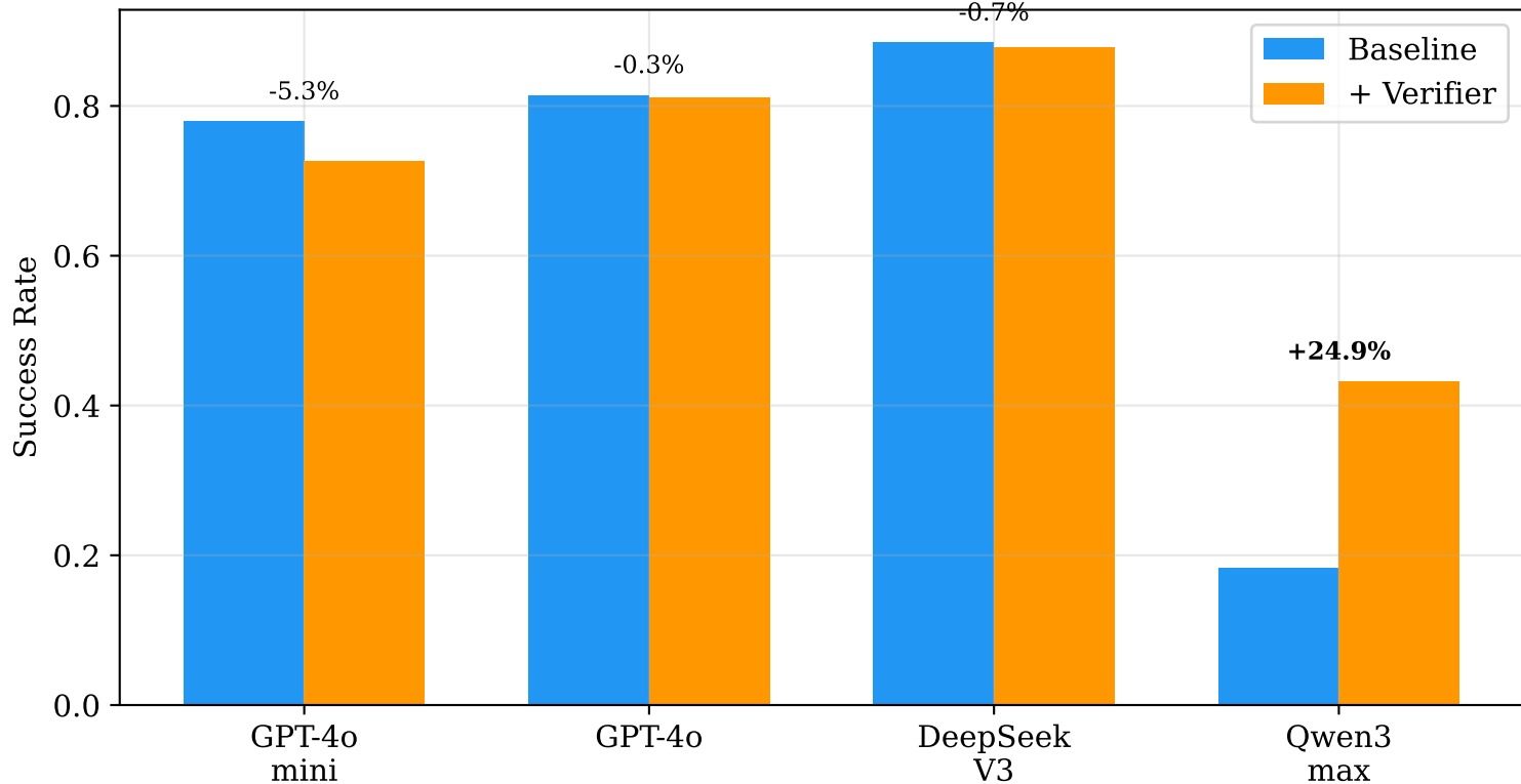
Verifier Ablation: Baseline vs +Verifier
