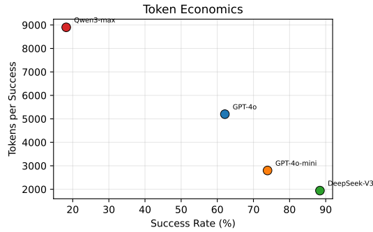
Figure 5: Tokens per success vs. success rate.
