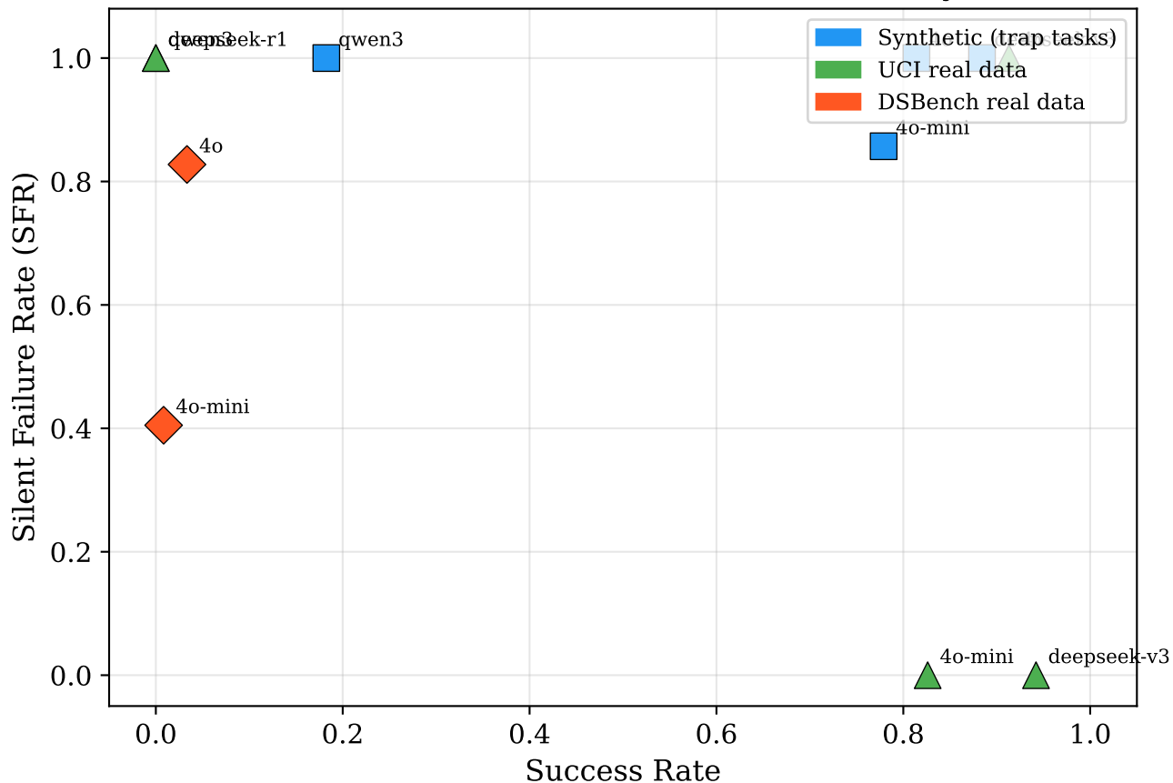
Failure Bifurcation: SFR vs Task Difficulty
