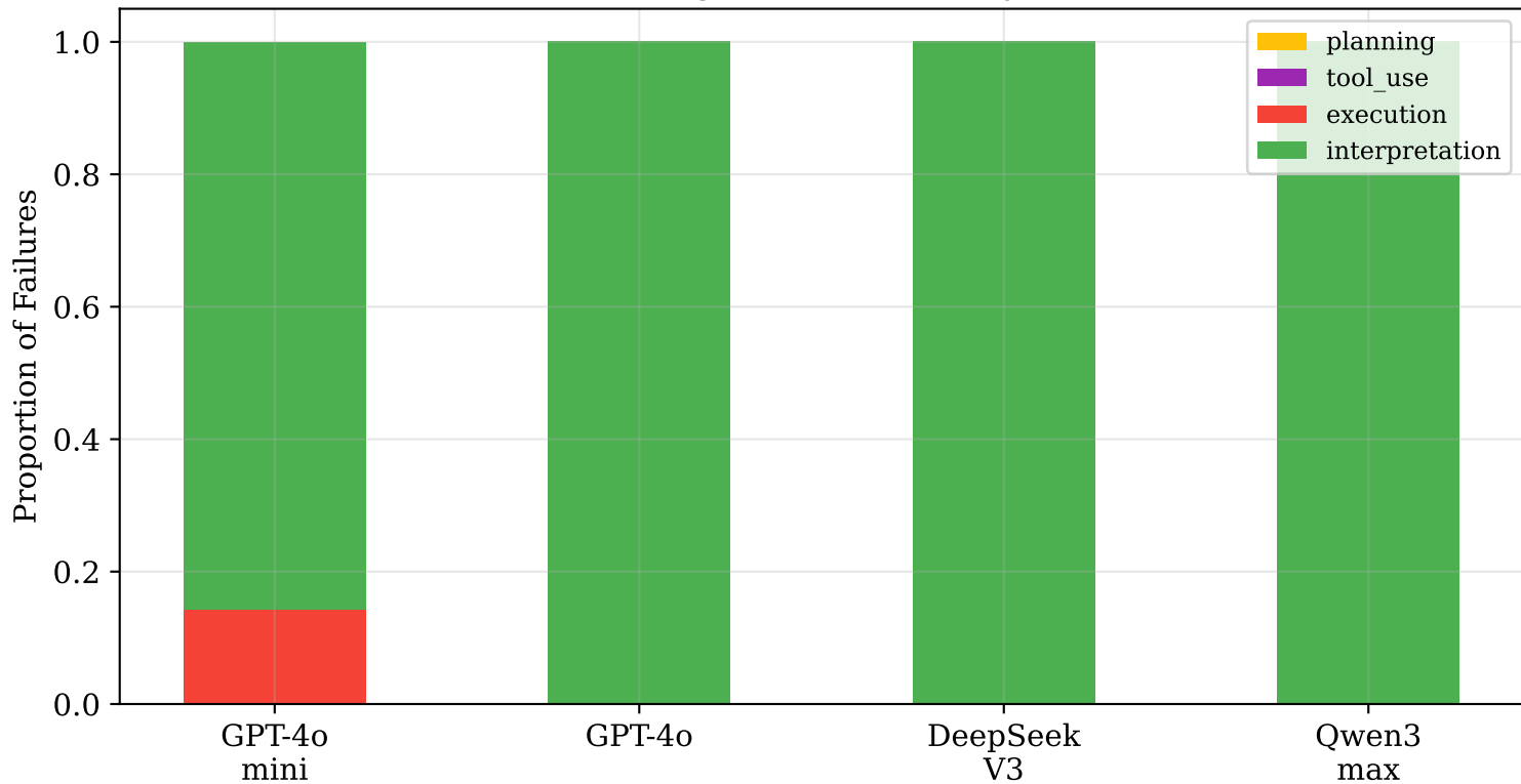
Failure Stage Distribution by Model
