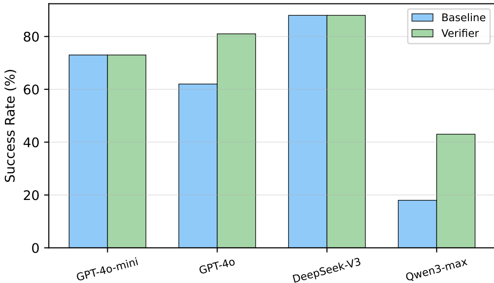
Verifier Ablation (Synthetic Tasks)
