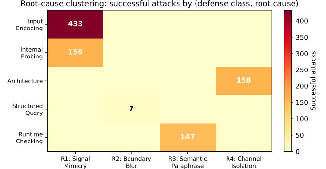
Fig. 3. Root-cause heatmap: each defense class has a single dominant failure mode.
