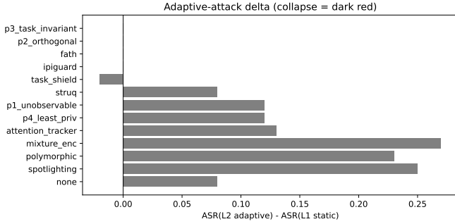
Fig. 4. Adaptive-attack delta: ASR(L2) – ASR(L1). Single-signal defenses show the largest increase.
