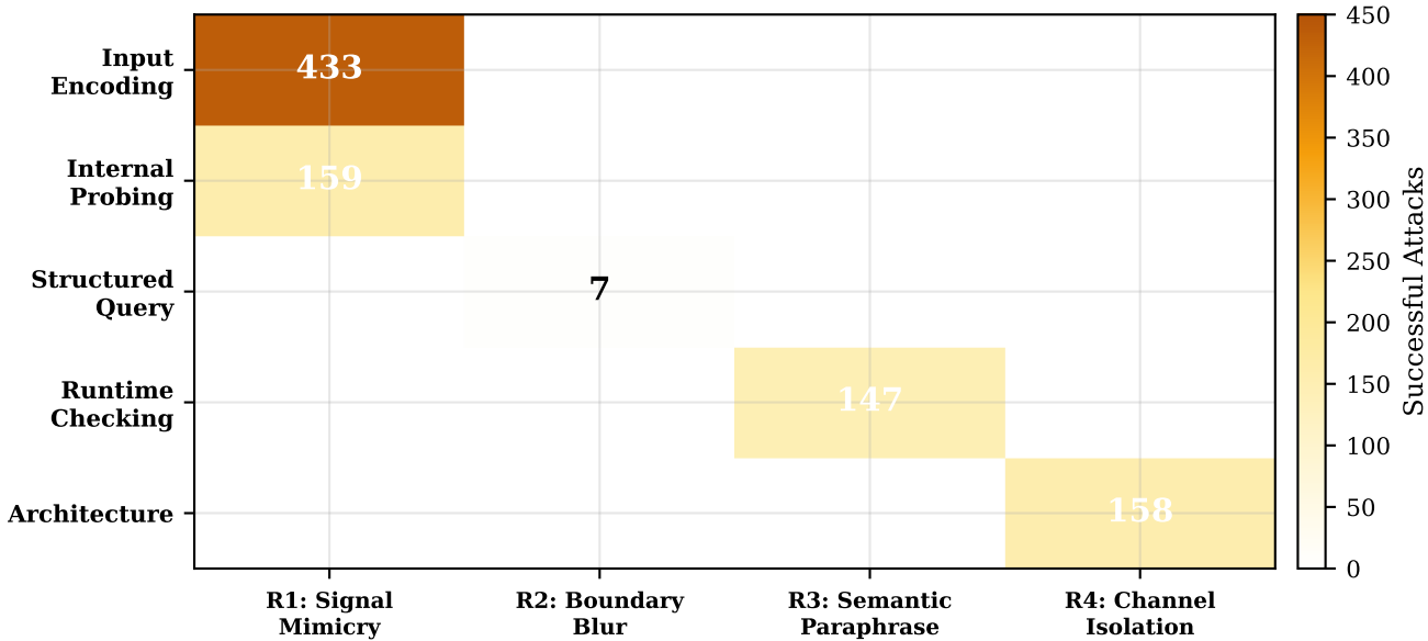
Root-Cause Clustering: Successful Attacks by (Defense Class, Root Cause)
