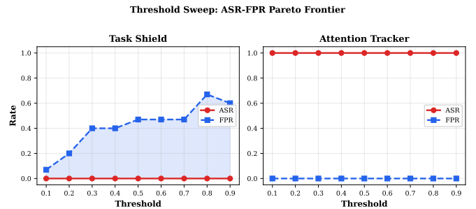
Fig. 2. Threshold sweep for Task Shield (left) and Attention Tracker (right). Task Shield’s FPR varies with threshold but ASR is always 0; Attention Tracker’s ASR is always 1.00 regardless of threshold.
