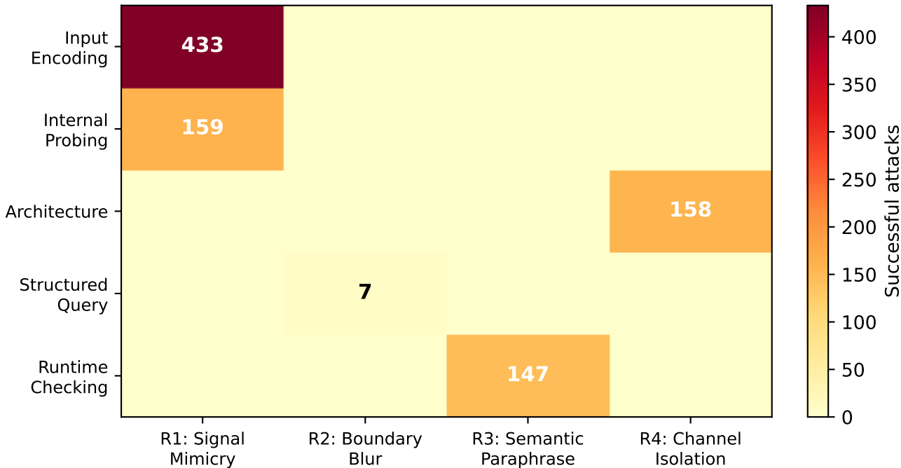
Root-cause clustering: successful attacks by (defense class, root cause)
