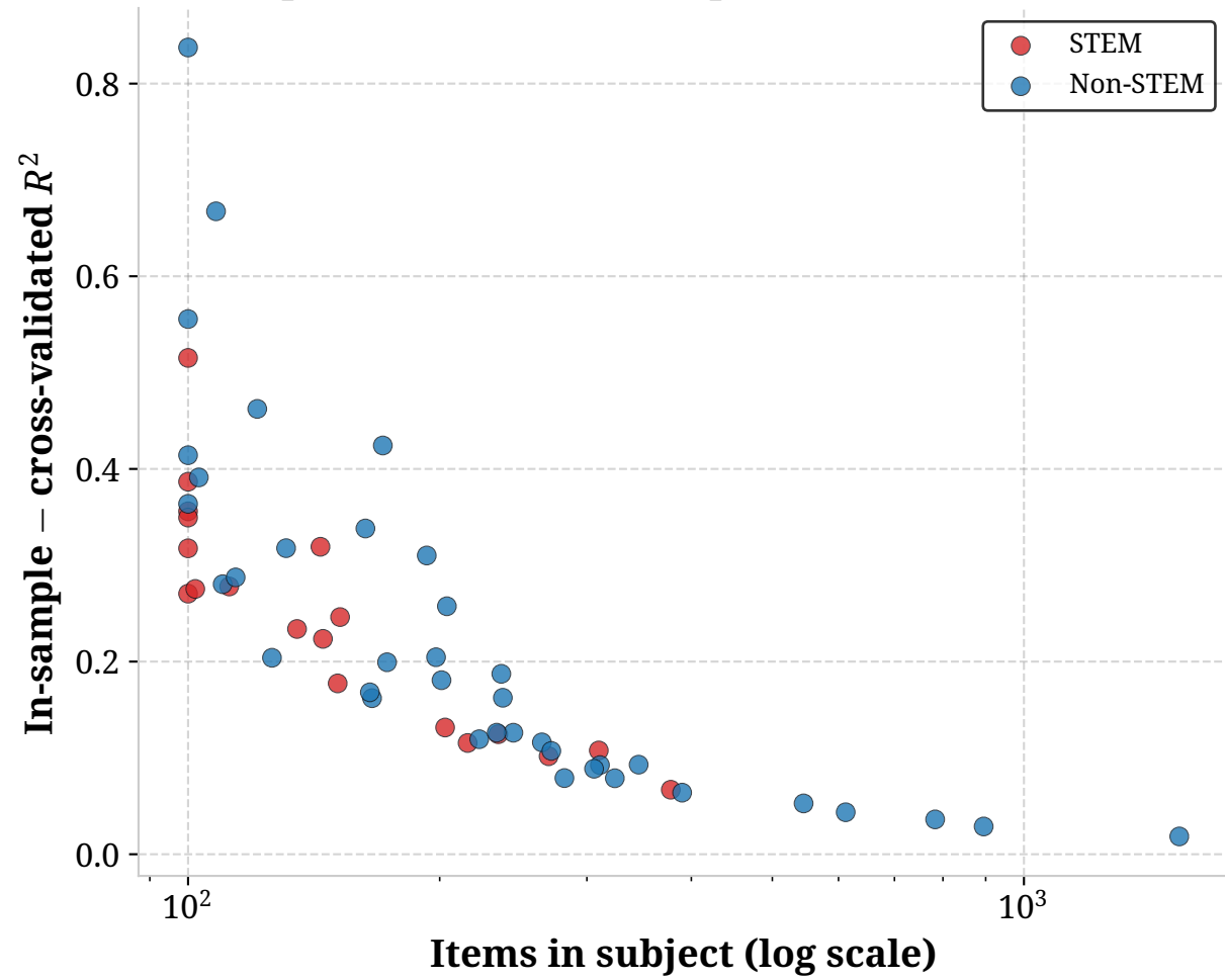
Optimism scales with the predictor-to-item ratio
