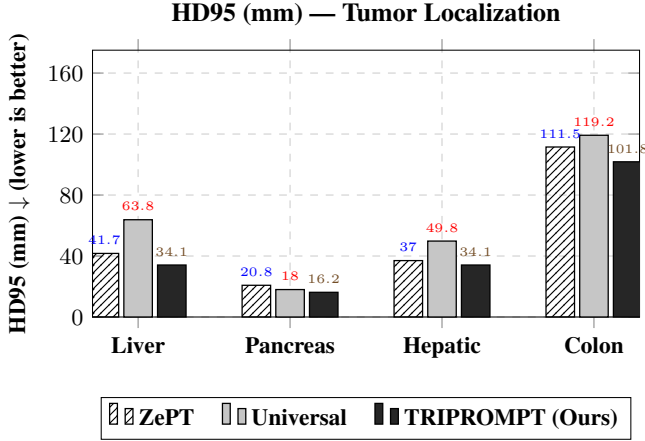
Figure 2: HD95 (mm) on tumor localization task. Lower is better. TRIPROMPT achieves the lowest boundary error across all four tumor classes. Colon HD95: 101.8 vs. 111.5 mm (ZePT), a reduction of 9.7 mm. Pancreas: 16.2 vs. 20.8 mm.
