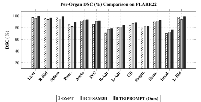
Figure 1: Per-organ DSC (%) on FLARE22 (all 13 classes). TRIPROMPT (solid black) achieves the highest DSC across all structures. Largest absolute gains over the best baseline: Pancreas (+4.6 pp), Duodenum (+3.7 pp), Gallbladder (+1.5 pp) — all high deformation-variability structures.
