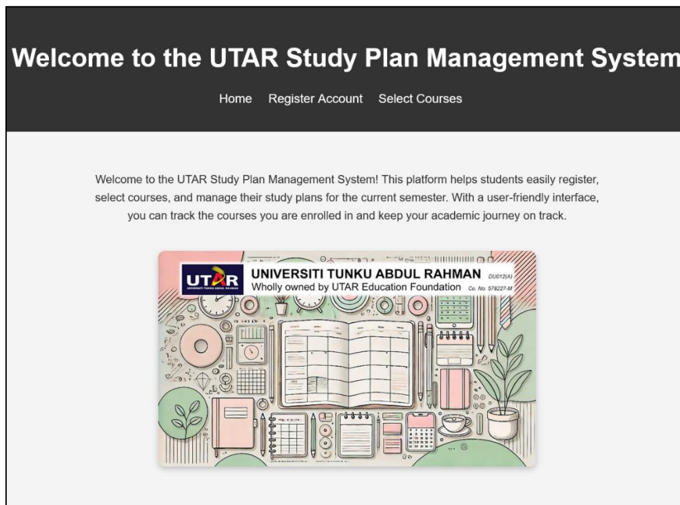
Figure 1: Homepage (index.php)
