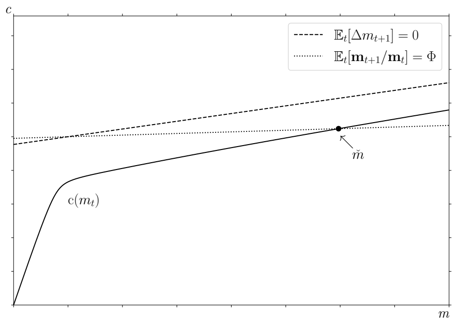
Figure 2 \{\text{FVAC}, \text{GIC}, \text{GIC-Mod}\} : No \hat{m} Exists But \tilde{m} Does
