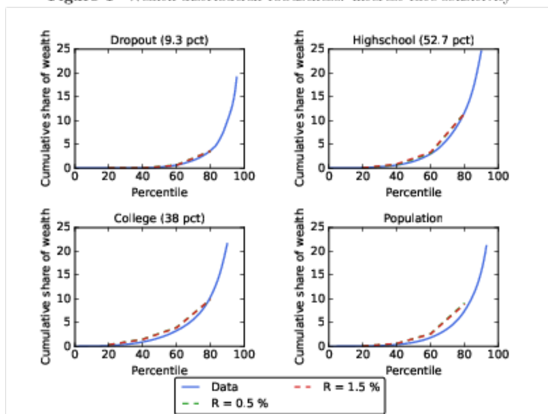
Figure 1 Wealth distribution robustness: interest rate sensitivity
