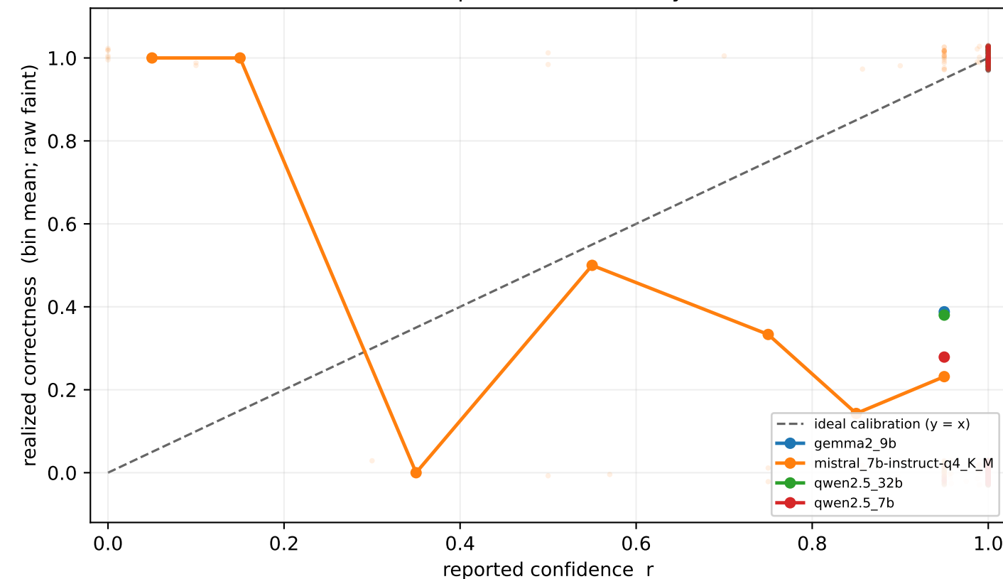
Panel 1 — per-model reliability (lead)
