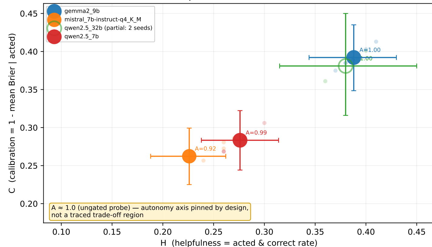
Panel 2 — (H, C) placement; A encoded as marker size
