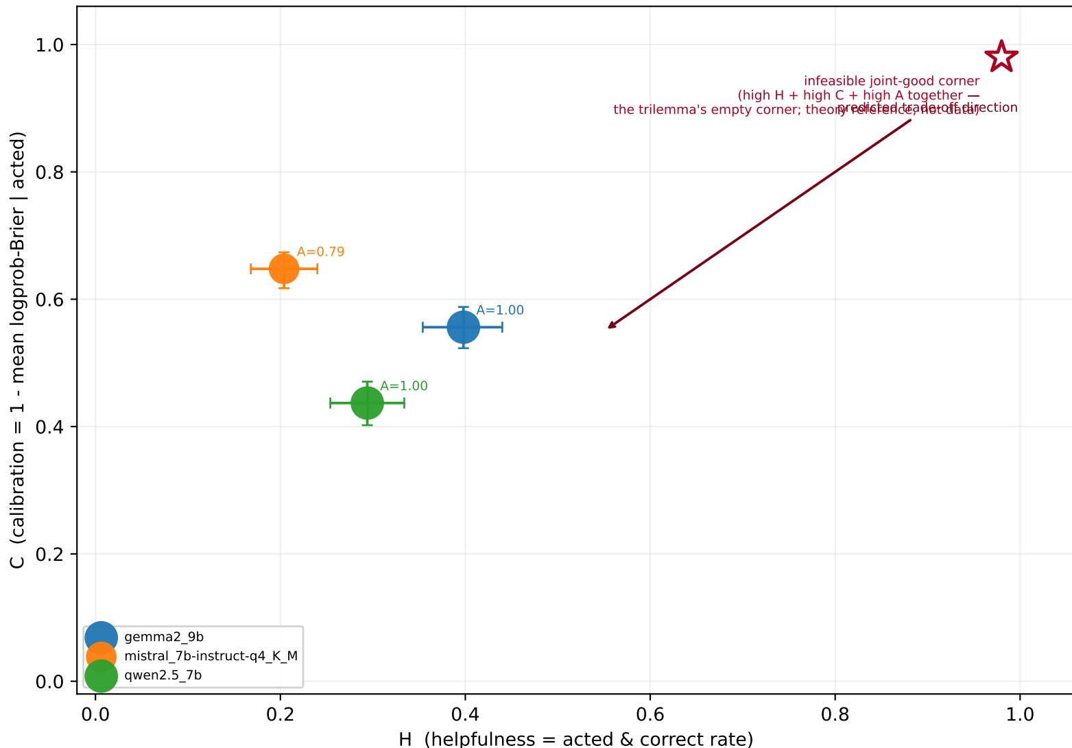
Logprob cross-model placement — (H, C); A as marker size
