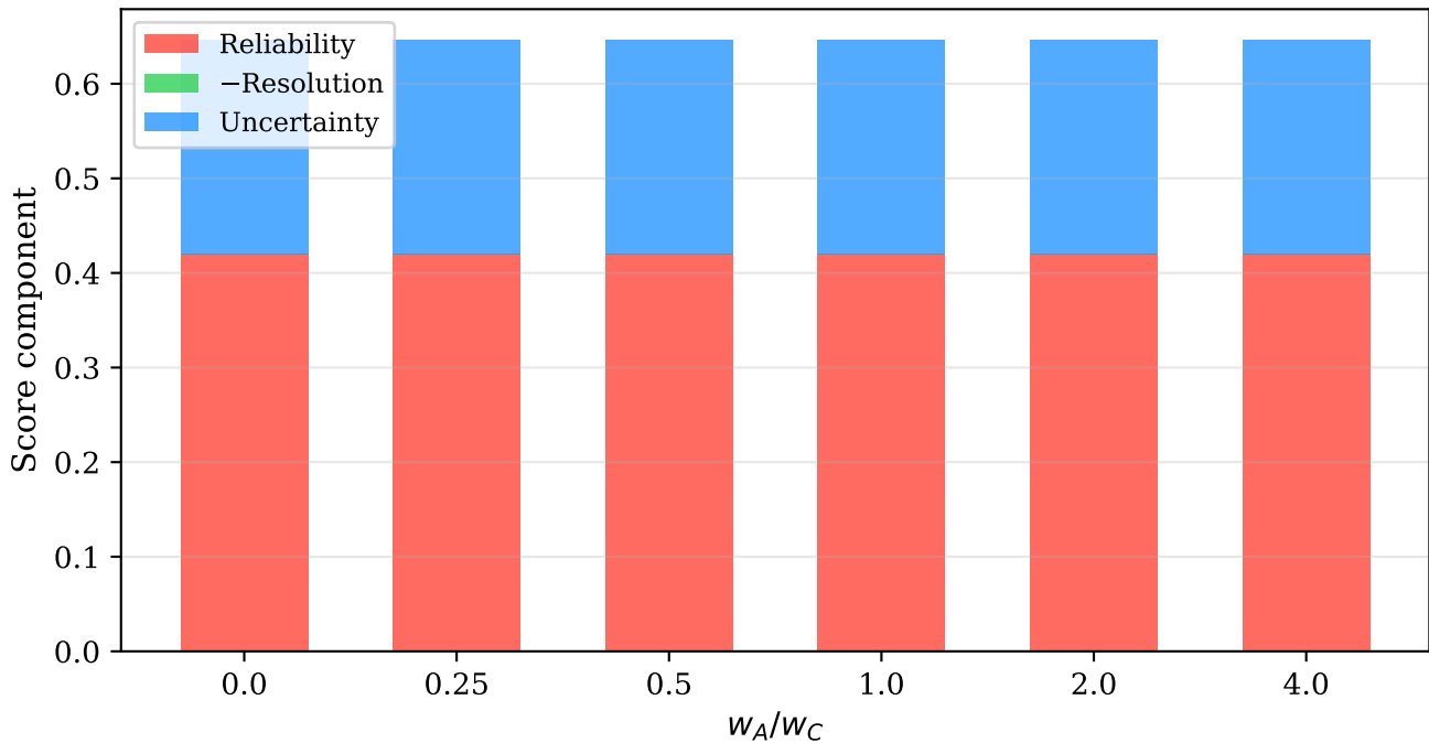
Brier decomposition ( N = 32 , r_{\min} = 0.9 )
