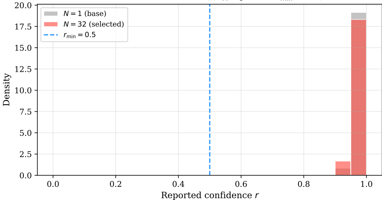
Confidence distribution ( w_A/w_C = 0.5 , r_{\min} = 0.5 )
