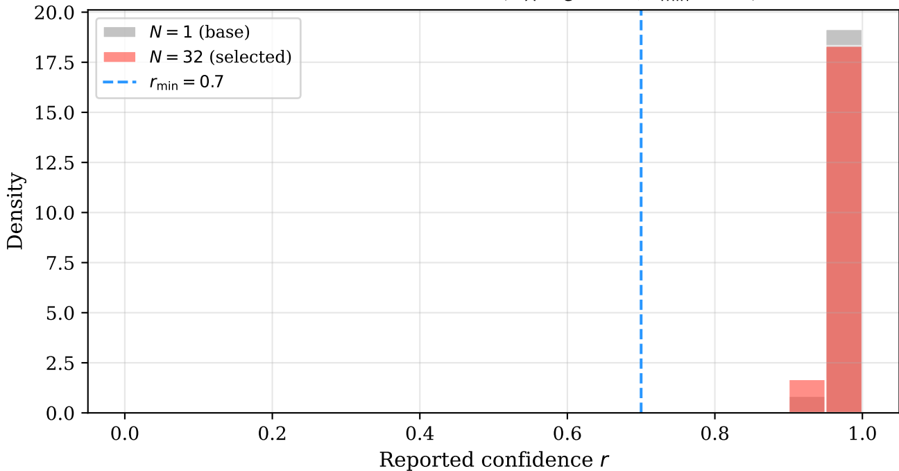
Confidence distribution ( w_A/w_C = 4.0 , r_{\min} = 0.7 )
