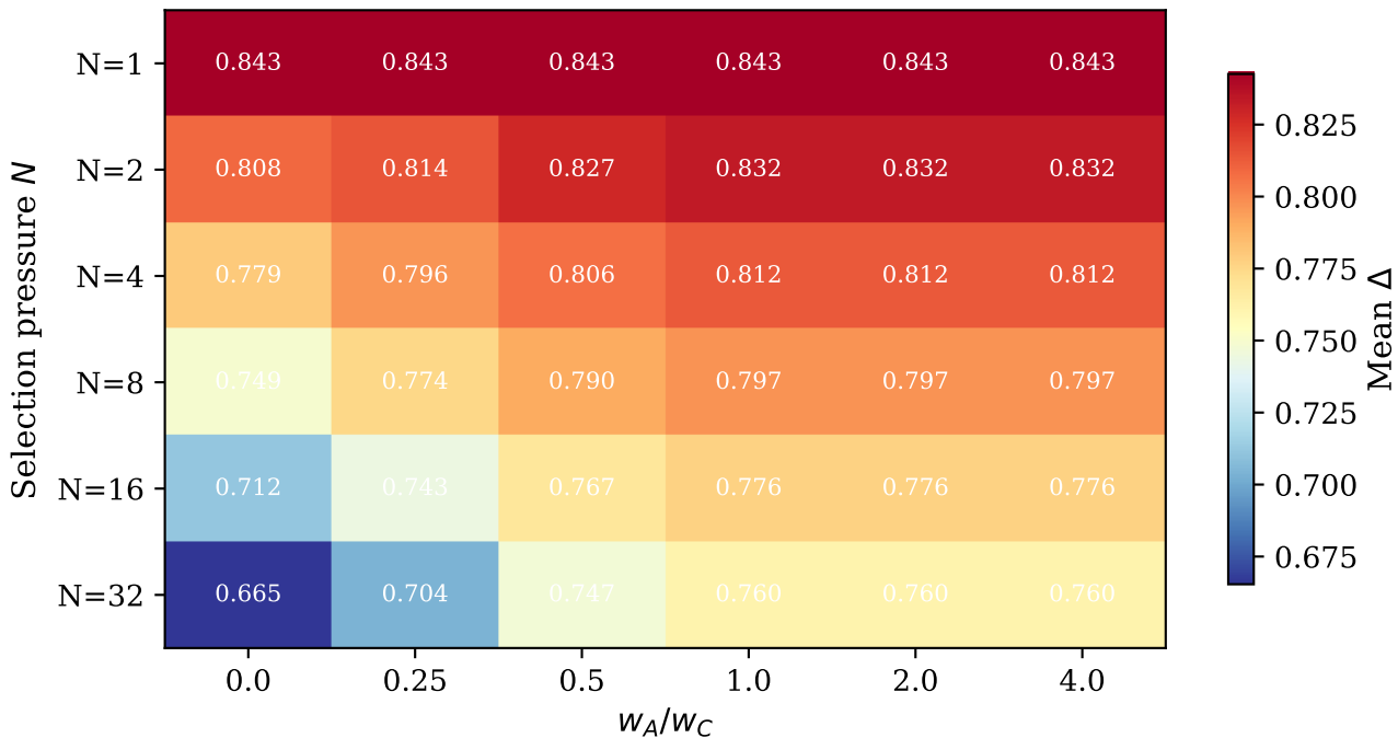
Mean confidence inflation on binding tasks ( r_{\min} = 0.7 )
