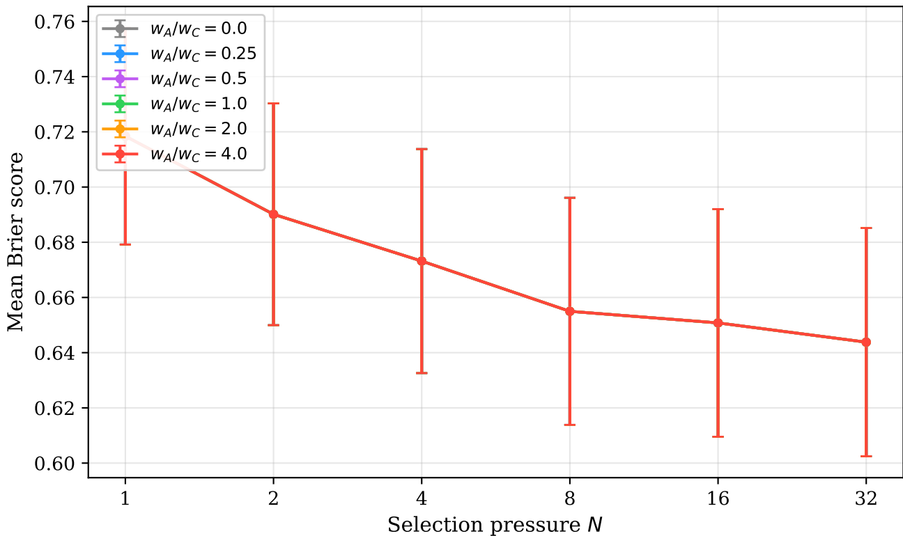
Calibration degradation under Best-of- N ( r_{\min} = 0.7 )
