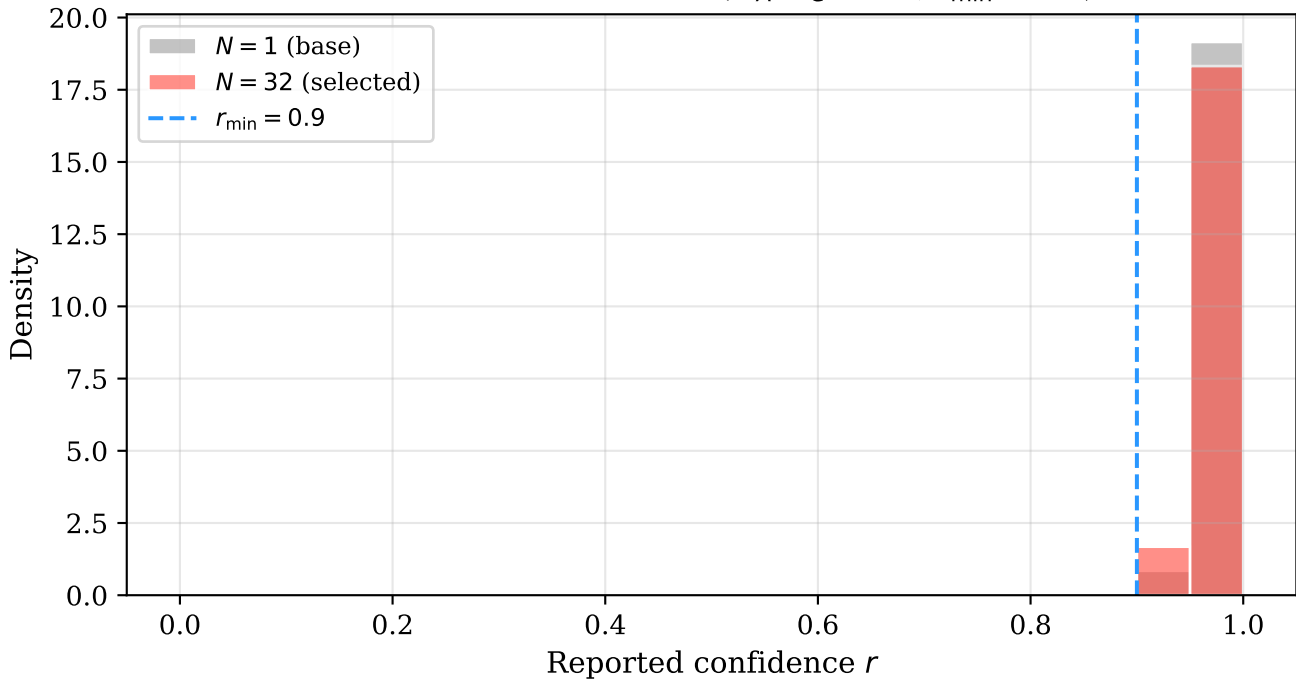
Confidence distribution ( w_A/w_C = 4.0 , r_{\min} = 0.9 )
